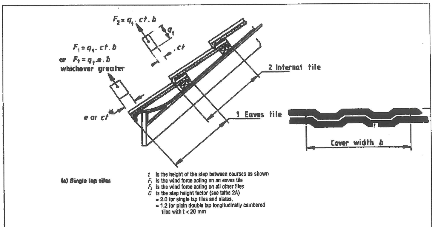
Figure 4. British Standard 5534.
