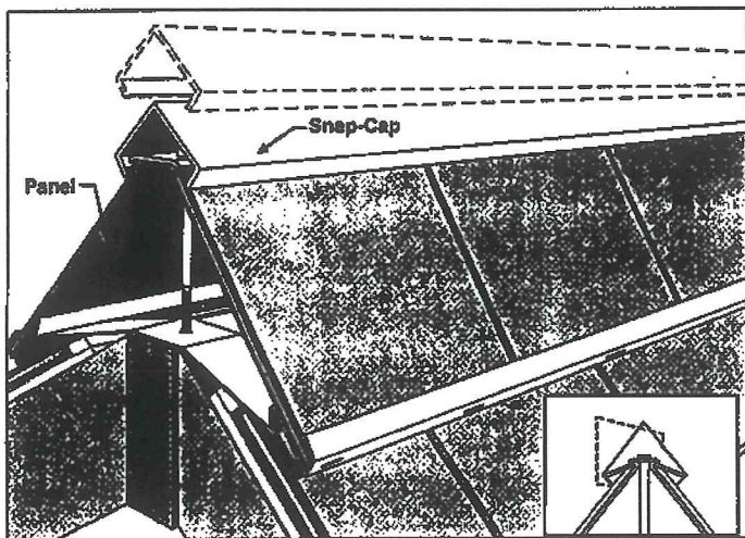
Figure 12. Ridge cap.
